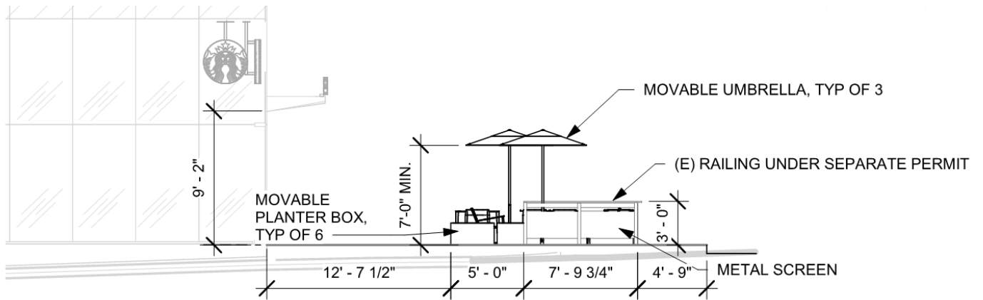
② SOUTH ELEVATION - FACING ASH 1/8" = 1'-0"
