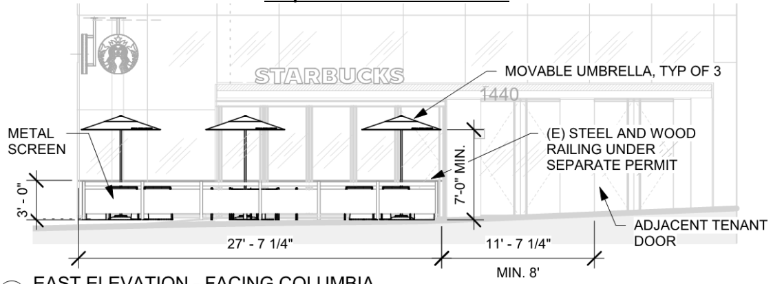
① EAST ELEVATION - FACING COLUMBIA 1/8" = 1'-0"
